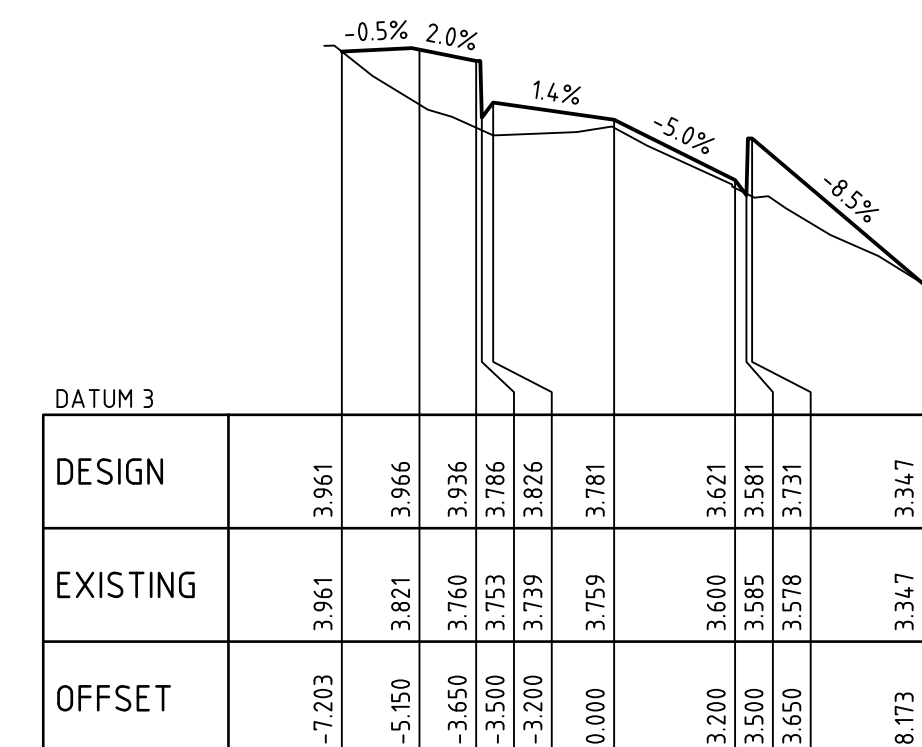
CHAINAGE 180.000
