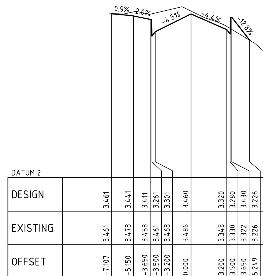
CHAINAGE 120.000
